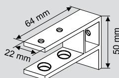
angular holder (with extra charge)
