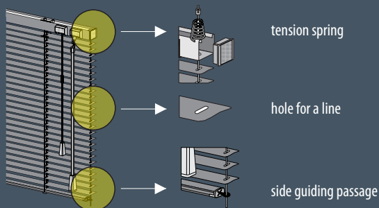
SIDE GUIDING
