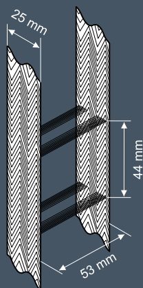
Laddertape 25 mm
