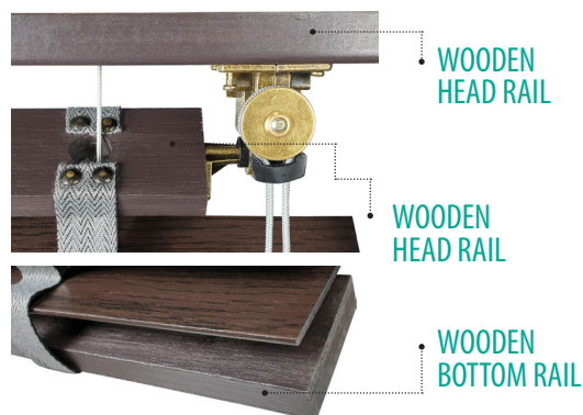
RETRO WOODEN BLIND 50 mm
