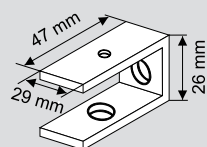
universal holder
