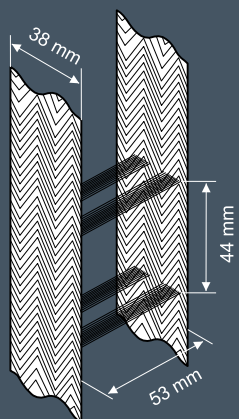
Laddertape 38 mm
