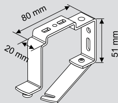
clamp (with extra charge)
