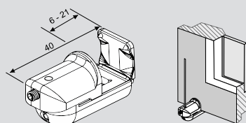
Clamp holder for non-invasive installation of the side guiding cord.
