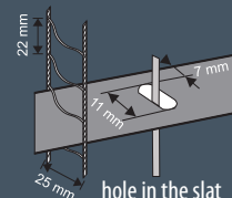
hole in the slat of standard blind
