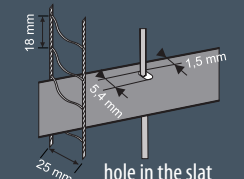
hole in the slat of BLACKOUT blind
